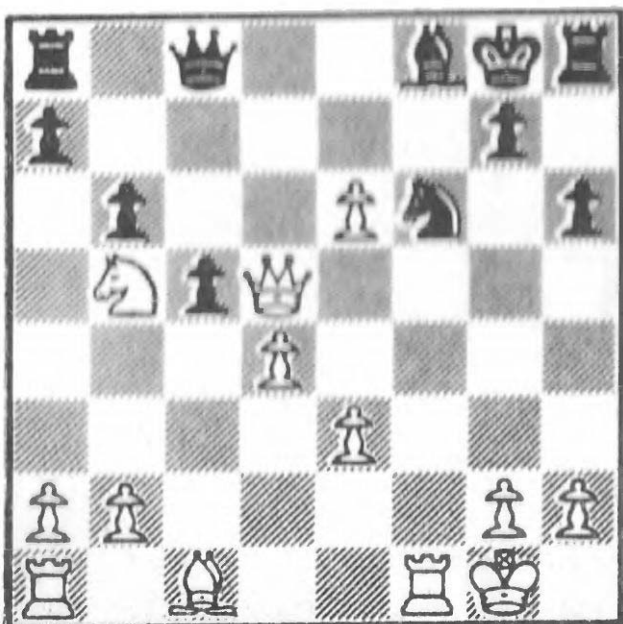
183 After 16...Nf6
